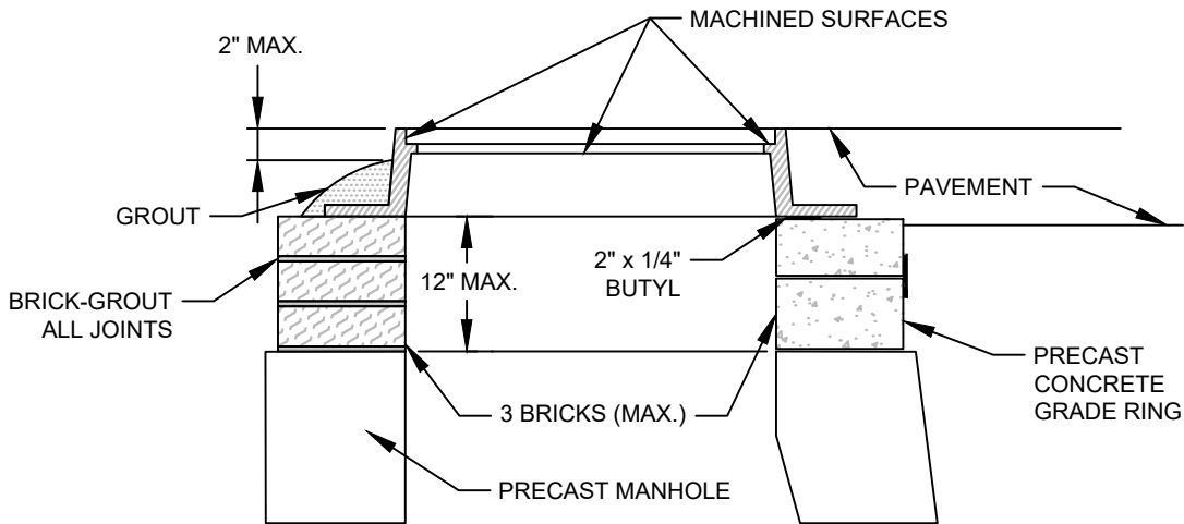
FRAME SET IN ROADWAY LOCATION N.T.S.
