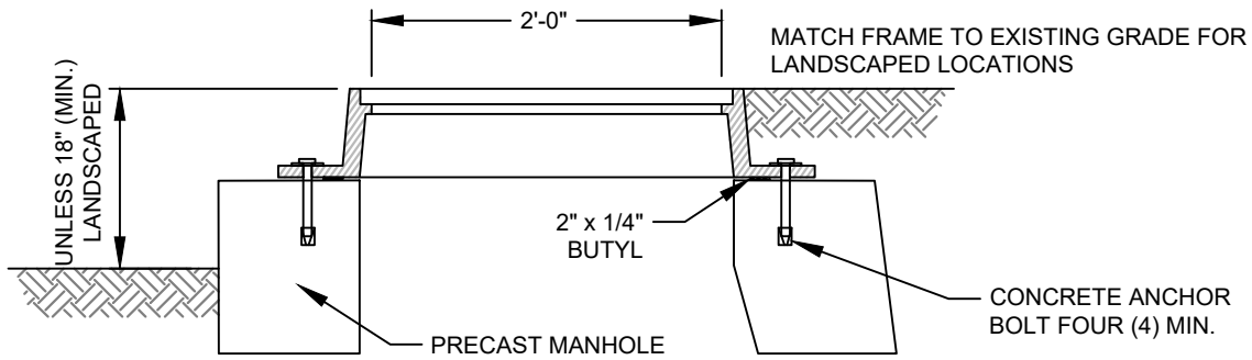
FRAME SET IN NON-ROADWAY LOCATION N.T.S.
