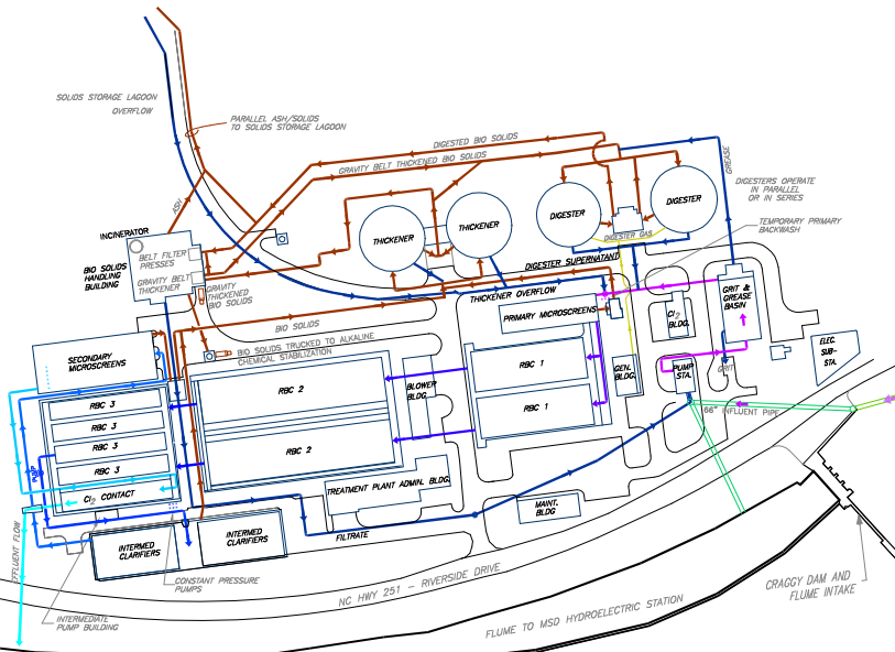
Treatment Plant Wastewater Flow
