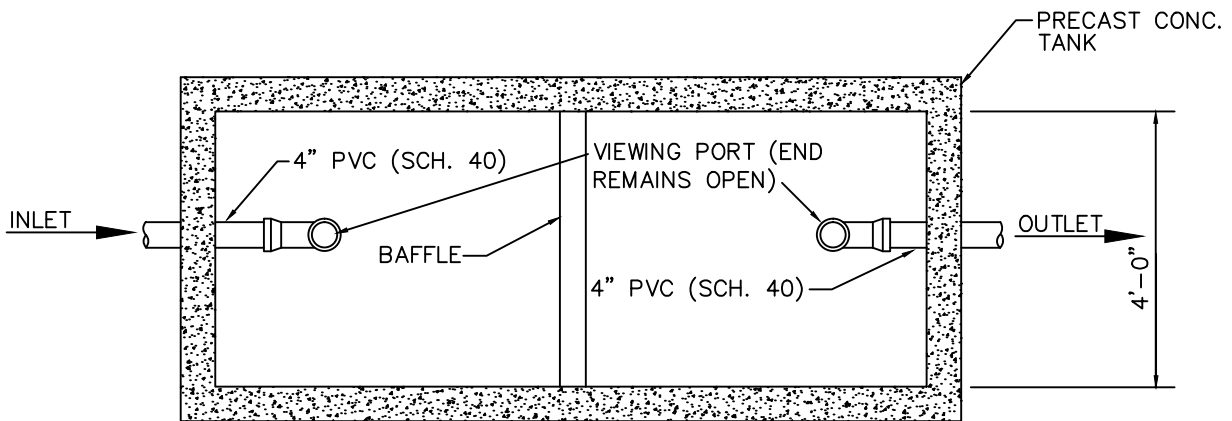
PLAN (OVERHEAD) VIEW
