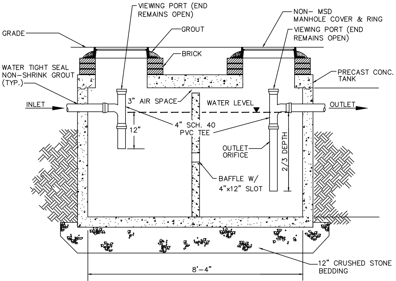
SECTION THRU GREASETRAP
