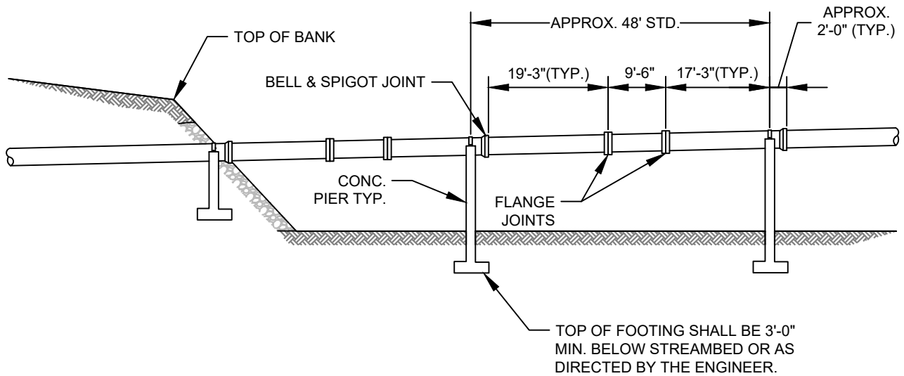
ELEVATED CROSSING - TYPE III (18" AND LARGER PIPE) N.T.S.
