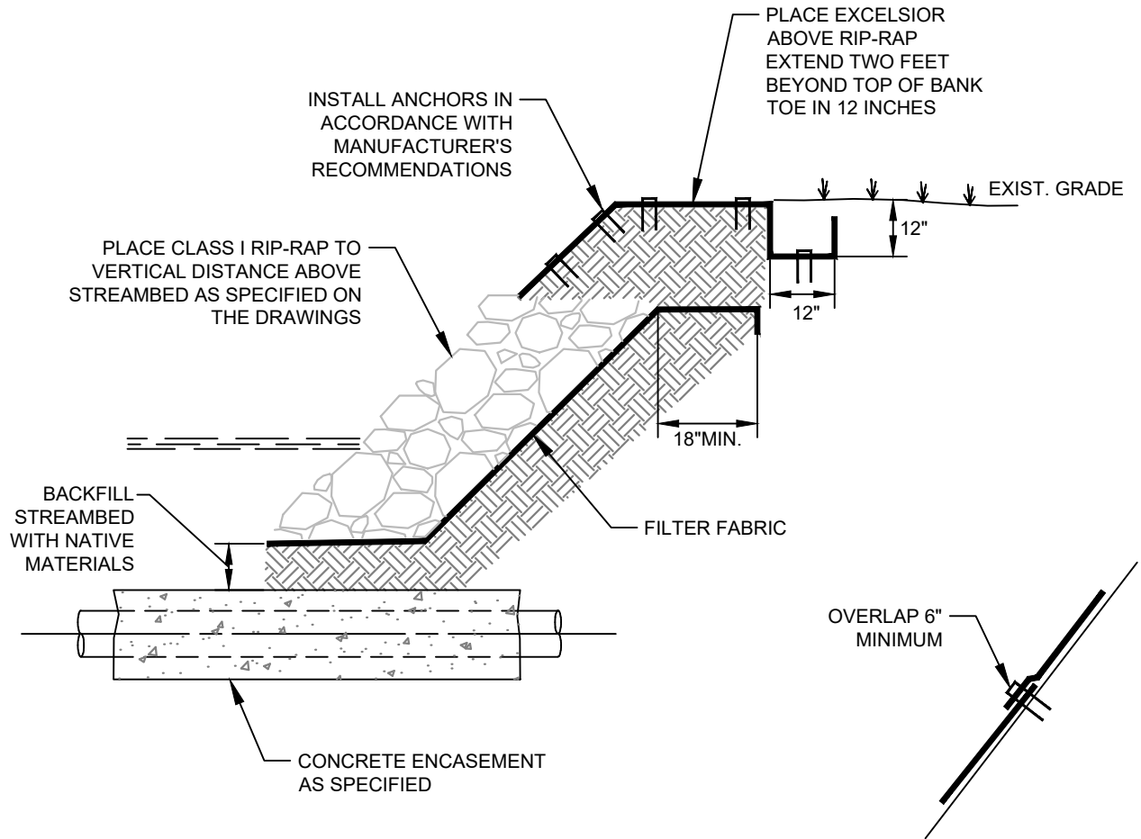
STREAMBANK RESTORATION DETAIL N.T.S.
